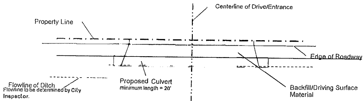
Front View
